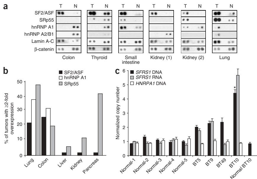
Figure 1 Upregulation and amplification of SF2/ASF in human tumors. (a) A protein microarray (Biochain) consisting of 47 pairs of tumor samples (T) and their normal tissue counterparts (N), spotted as duplicates, was probed with the indicated antibodies. Representative tumor samples overexpressing SF2/ASF and corresponding controls: colon, adenocarcinoma; thyroid, follicular carcinoma; small intestine, leiomyoma; kidney (1), clear cell carcinoma; kidney (2), granular cell carcinoma. (b) Expression of splicing factor mRNA was measured by reverse-transcription quantitative PCR (RT-qPCR) in 50 tumor samples and five normal samples from each indicated tissue and normalized to \beta -actin mRNA. Bars show the proportion of tumors overexpressing the mRNA more than two-fold over the mean of the five normal samples. Expression of hnRNP A1 was determined only in lung and colon tumors. (c) DNA and RNA were measured by qPCR and RT-qPCR in 50 breast tumor samples and five normal samples. Data for the four tumors (infiltrating ductal carcinomas) with elevated DNA copy numbers of SF2/ASF are shown relative to the mean of the normal samples. Normal BT10, surrounding normal breast tissue from the patient with the BT10 tumor. Means \pm s.d. from triplicate qPCR measurements are shown. *P = 4.9 \times 10^{-10} for the BT10 versus normal BT10 comparison; n = 6 .
