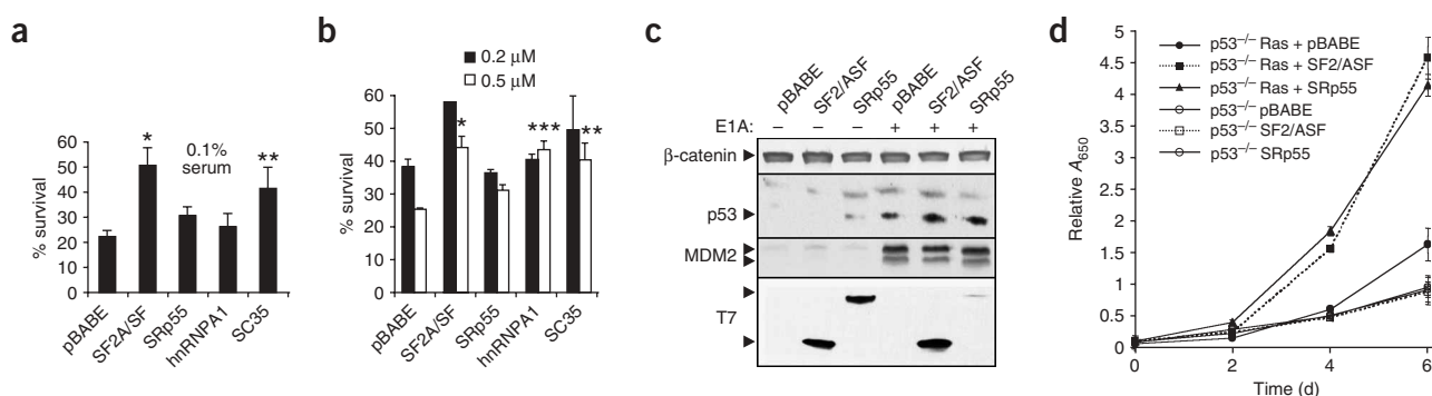
Figure 3 SF2/ASF overexpression protects E1A-sensitized MEF cells against apoptosis and enhances the proliferation of Ras-transformed cells. Primary wild-type MEF cells were transduced with retroviruses expressing the indicated human splicing factor cDNAs, or with the empty vector; some cells were cotransduced with adenovirus E1A or activated Ras, as indicated. Error bars indicate s.d. (a) After drug selection, cells coinfecting with E1A were plated and serum-starved, and cell death was measured by trypan blue staining. P -values in pairwise comparisons to the pBABE control: * P = 5 \times 10^{-8} ; ** P = 5 \times 10^{-5} ; n = 3. (b) Cells coinfecting with E1A were plated and treated with the indicated adriamycin concentrations after 24 h, and cell death was measured as in a . * P = 0.003, ** P = 0.01, *** P = 0.006; n = 3; for SF2/ASF at low adriamycin, n = 1. (c) MEF cells were infected with the indicated retroviruses, plated after single or double selection ( 10^6 cells per 10-cm plate) and lysed in SDS after 24 h. Western blots were carried out using the indicated primary antibodies. The reduction in SRp55 in the presence of E1A was not observed with other cell lines (data not shown). (d) p53 -/- MEF cells were transduced with the empty vector or with retroviruses expressing SF2/ASF or SRp55, either alone or with oncogenic Ras. Cells were fixed at 48-h intervals and stained with methylene blue. Each point represents the mean relative absorbance from six wells.
