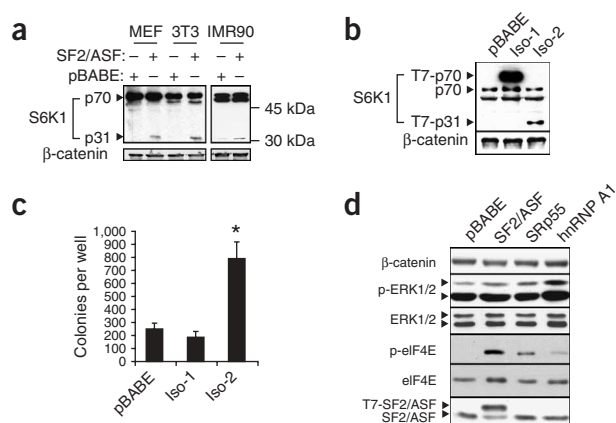
Figure 5 SF2/ASF promotes expression of an oncogenic isoform of S6K1 and induces eIF4E phosphorylation. (a) MEF, NIH 3T3 and IMR90 cells were transduced with pBABE or SF2/ASF retroviruses and lysed in SDS. Western blotting was carried out using a monoclonal antibody against the N terminus of S6K1 to detect the endogenous isoforms and one against \beta -catenin as a loading control. (b) NIH 3T3 cells were transduced with pBABE or S6K1 isoform-1 or isoform-2 retroviruses, and lysates were analyzed by western blotting as in a . The S6K1 antibody reacts with both the endogenous and T7-tagged S6K1 isoforms, but the endogenous isoform-2 is not detected in this exposure. (c) Aliquots of cells in b were seeded in soft agar, and colonies were counted 14 d later. Means \pm s.d. are shown; * P = 6 \times 10^{-7} compared to the pBABE control. (d) MEF cells were transduced with the indicated retroviruses and analyzed by western blotting with the indicated antibodies.
