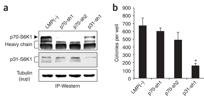
Figure 7 Knockdown of S6K1 isoform-2 blocks SF2/ASF-mediated transformation. (a) Immunoprecipitation (IP)-western blot analysis of S6K1 isoforms in NIH 3T3 cells overexpressing SF2/ASF, after transduction with retroviruses expressing the indicated S6K1 isoform-specific shRNAs. (b) Cells described in a were seeded in soft agar and colonies were counted as in Figure 6b ; means \pm s.d. are shown. * P = 6 \times 10^{-8} .
