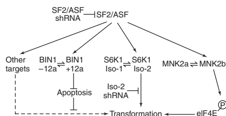
Figure 8 A model for transformation by SF2/ASF. SF2/ASF (which can be blocked by specific shRNAs) activates several key targets that contribute to the transformed phenotype: induction of MNK2b promotes phosphorylation of eIF4E, which enhances cap-dependent translation; induction of the oncogenic S6K1 isoform-2 directly leads to transformation; and induction of inactive isoforms of the putative tumor suppressor BIN1 inhibits apoptosis. Other SF2/ASF targets are also likely to contribute to transformation.
