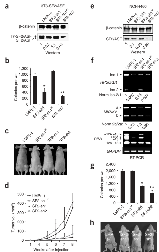
Figure 6 Knockdown of SF2/ASF reverses transformation of NCI-H460 cells and SF2/ASF-overexpressing NIH 3T3 cells. (a) Western blot analysis of SF2/ASF in NIH 3T3 cells overexpressing SF2/ASF after transduction with viruses expressing the indicated SF2/ASF shRNAs. The SF2/ASF-specific shRNAs target the 3' UTR of SF2/ASF and therefore affect only the endogenous SF2/ASF (lower band), for which normalized protein levels are shown under the blot. SF2-sh1 m is a control shRNA with two mismatches. (b) Cells described in a were seeded in soft agar, and colonies were counted 14 d later; means \pm s.d. are shown. P -values for comparisons to the LMP(-) control: * P = 2 \times 10^{-7} ; ** P = 2 \times 10^{-9} . (c,d) Cell lines described in a were injected into nude mice ( n = 8 injections) and tumor volume was measured weekly; error bars indicate s.d. Representative mice are shown. (e) Western blot of total protein from NCI-H460 cells as in a . (f) RNA from the cells in e was analyzed by RT-PCR and RT-qPCR to detect MKNK2 , RPS6KB1 and BIN1 isoform levels, with GAPDH as a control. Normalized ratios of RPS6KB1 isoform-2 to isoform-1 and MKNK2 2b to 2a calculated from the RT-qPCR data are shown under the corresponding gels. (g) Soft agar colony formation by cells described in e . Means \pm s.d. are shown. P -values calculated as in b : * P = 3 \times 10^{-11} ; ** P = 2 \times 10^{-15} . (h) Cell lines described in a were injected into nude mice ( n = 8 injections). Representative mice are shown.
