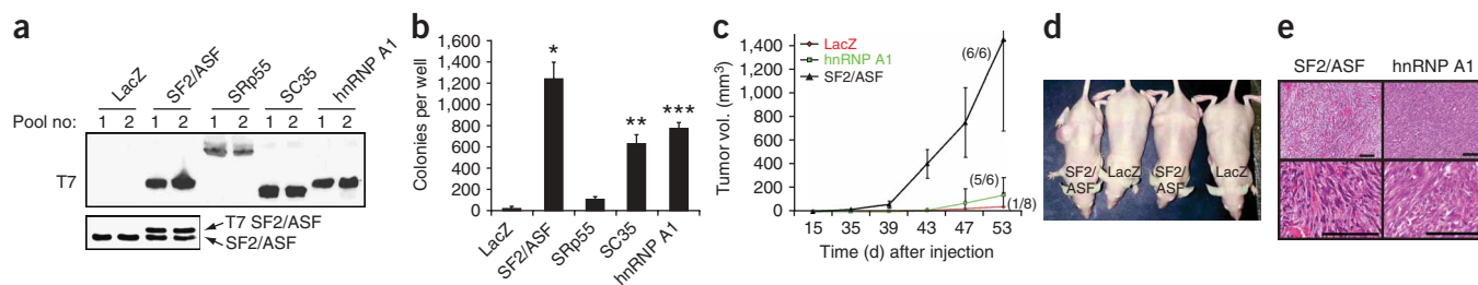
Figure 2 SF2/ASF transforms immortal cells and is tumorigenic in nude mice. (a) Total proteins from duplicate pools of NIH 3T3 stable cell lines transduced with retroviruses expressing LacZ or T7-tagged SF2/ASF, SRp55, SC35 or hnRNP A1 were analyzed by western blotting with anti-T7. The first four samples were also analyzed with anti-SF2/ASF (below) to compare the expression of endogenous and transduced SF2/ASF. (b) Quantification of soft-agar colony formation by the stably transduced cell lines. The mean \pm s.d. for each pair of pooled lines is shown. P -values in pairwise comparisons to the LacZ control: * P = 4 \times 10^{-8} ; ** P = 10^{-7} ; *** P = 7 \times 10^{-8} . (c) Tumor growth curve in mice injected with 2 \times 10^6 cells from the indicated NIH 3T3 pooled lines. The number of tumors formed per number of injections is shown in parentheses. SRp55 and SC35 cell lines (six each) did not form tumors during the same time course (data not shown). Error bars, s.d. (d) Representative mice injected with LacZ-expressing control cells, or with SF2/ASF-overexpressing cells. (e) Light micrographs of formalin-fixed, paraffin-embedded tissue sections from tumors derived from NIH 3T3 cells overexpressing SF2/ASF or hnRNP A1, stained with hematoxylin and eosin. Scale bars, 100 \mu m.
